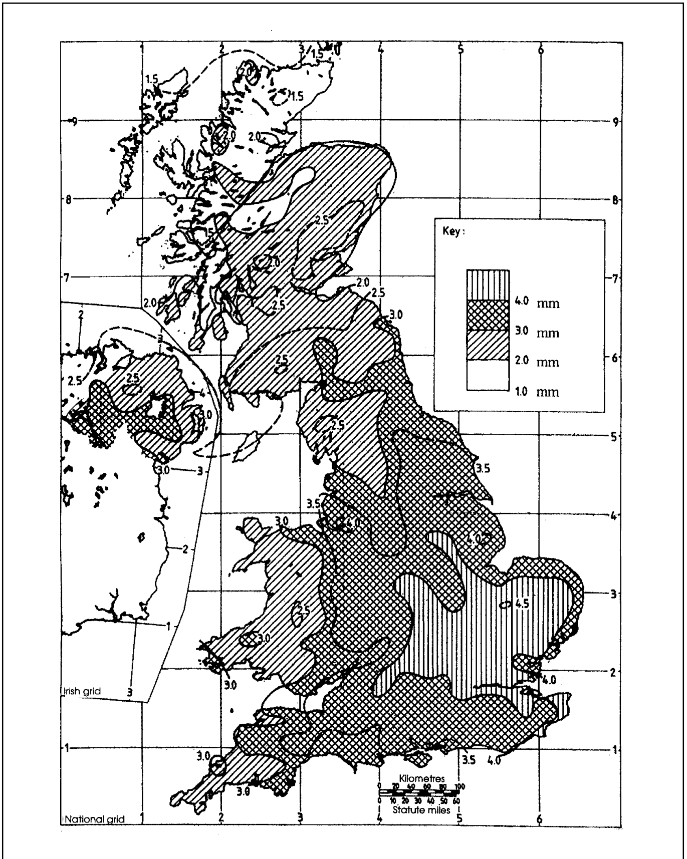
Figure 3 Values of 2minM5 rainfall depth for the UK (Reproduced from BS6367:1983, as amended, by permission of the British Standards Institution)
