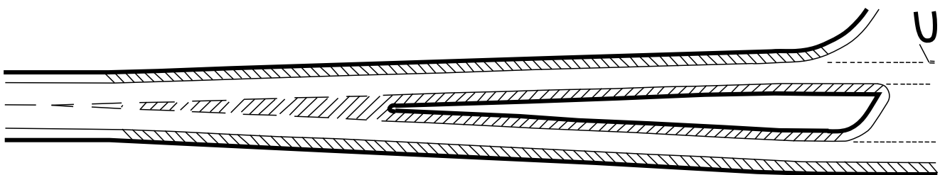
Figure 3/1 : Use of Hatching in Metre Strips to Eliminate Overtaking Manoeuvres (para 3.2)
