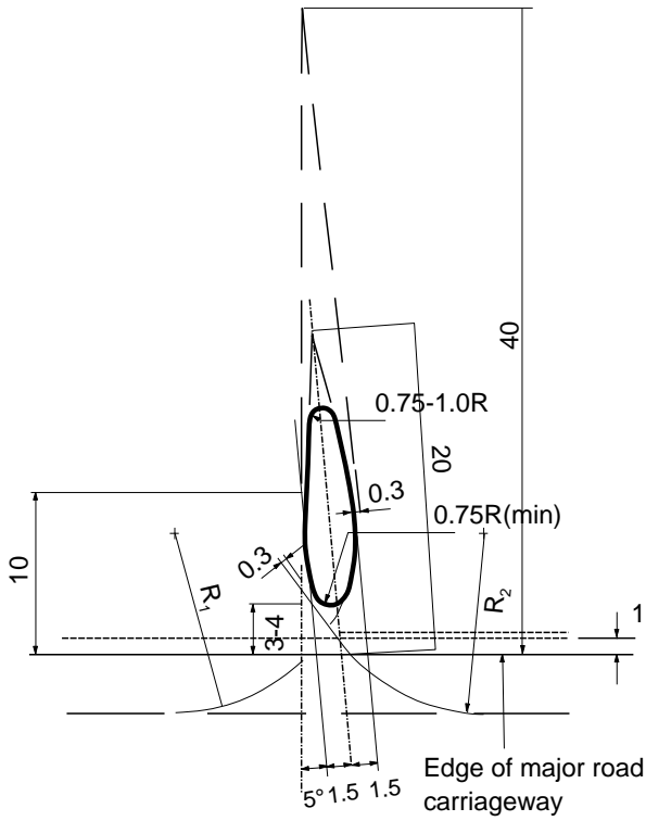
Figure A2/2 : Design of Rural Crossroads Channelling Island ( Dimensions in metres )
