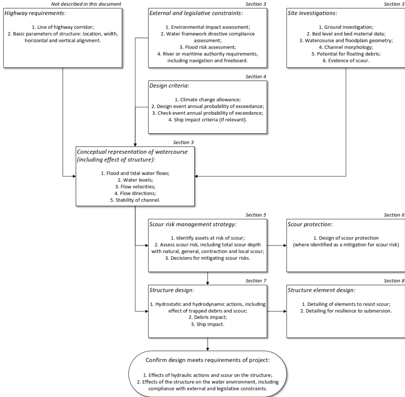
Figure 2.1N2 Summary of design procedure
