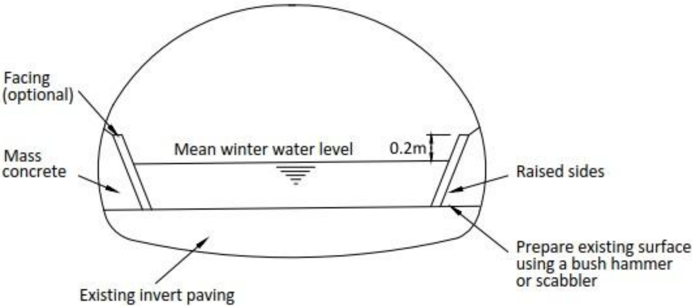
Figure B.4 Extension of an invert paving
