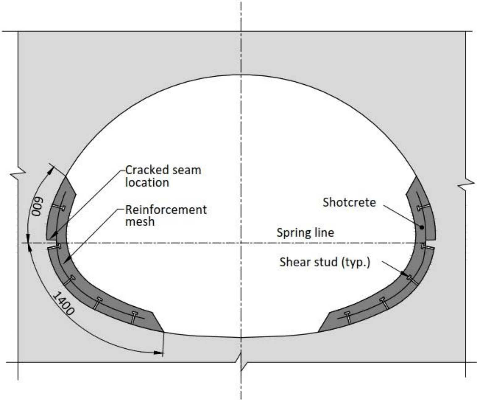
Figure B.13 Shotcrete reinforced concrete paving (after Abdel-Sayed et al, 1993)
