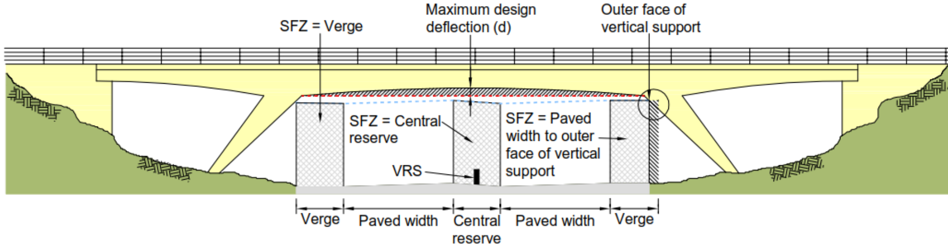
Figure 4.6N1 Minimum width of the SFZ
