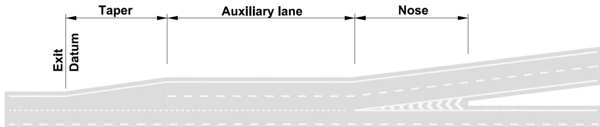
Figure 3.30i Layout E - 2-lane drop
