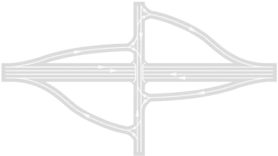
Figure A.1 Typical layouts of grade separated junctions - diamond
