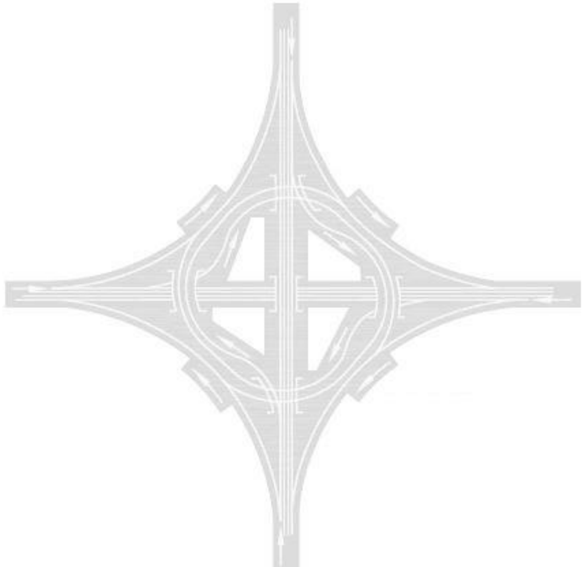
Figure A.8 4-way, 2-level cyclic interchange
