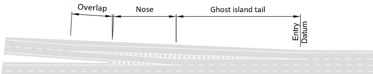
Figure 3.14h Layout F - 2 lane gain with ghost island
