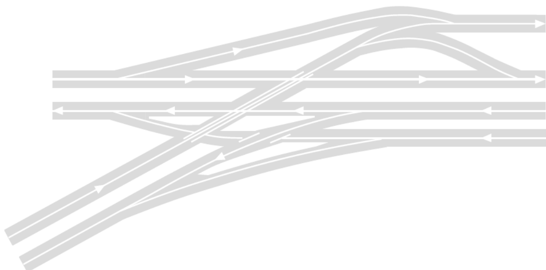
Figure A.14 3-leg 'Y' interchange of 2 motorways with mainline motorway and link roads
