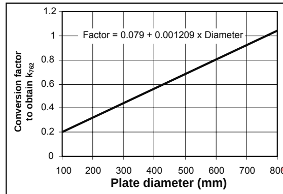
FIGURE 7.4 Conversion Factors for Smaller Plate Sizes
