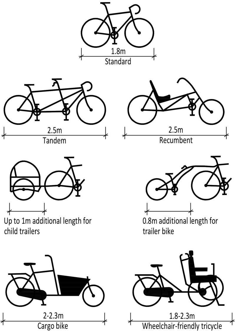
Figure E/2.1N3 Categories of cycle
