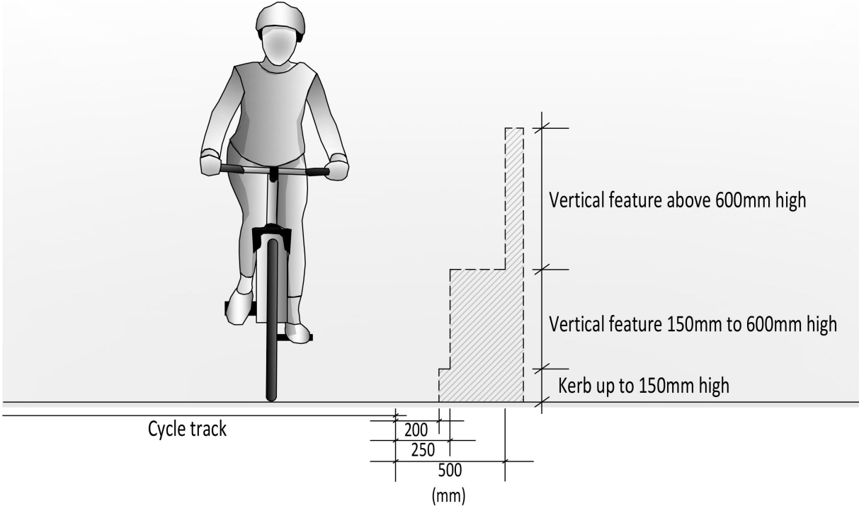
Figure E/3.2N Additional width required to maintain effective width of cycle tracks
