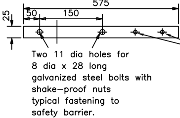
TYPES 8 FIXING STRAP (Bracket)
