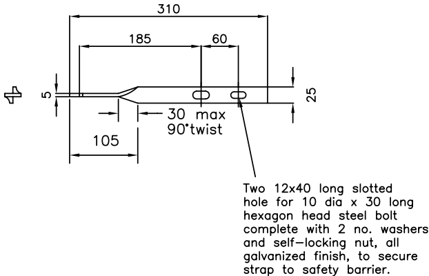
TYPE 9A FIXING STRAP (Bracket)
