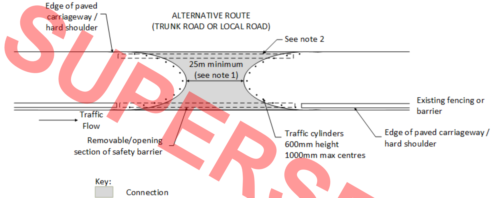
Figure E/A.3 Connection to parallel alternative road
