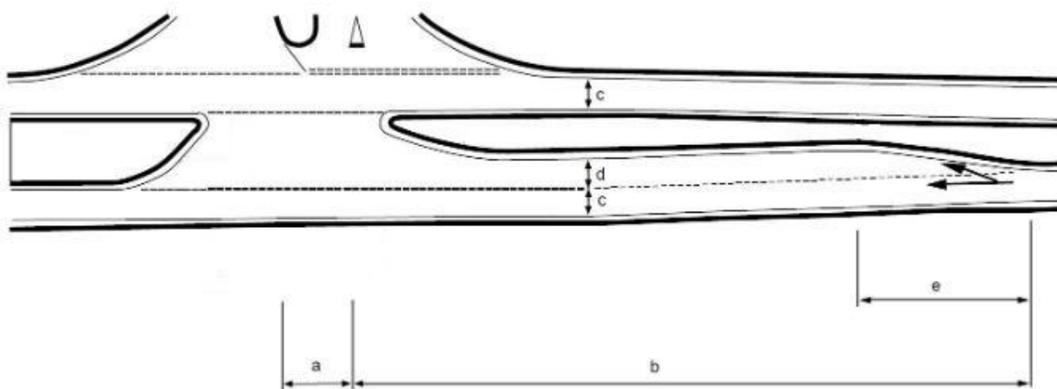
Figure 6.3d Major / minor priority junctions with SLD
