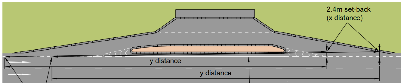
Figure 3.16 Visibility requirements at the exit from type A parking lay-bys with a merge taper
