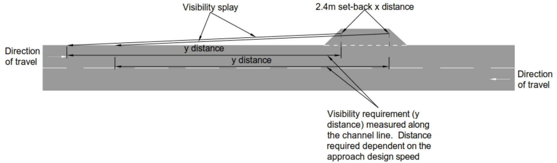
Figure 3.17Nb Visibility requirements at the exit from a type B parking lay-by - nearside lane
