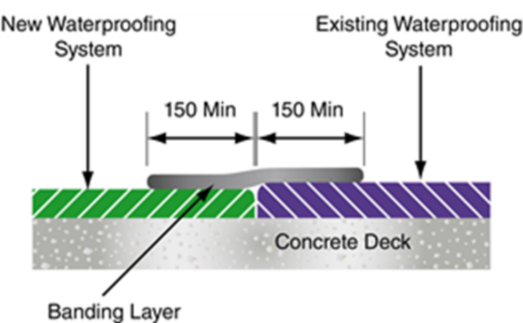
Figure D.1 Overlapping other waterproofing systems
