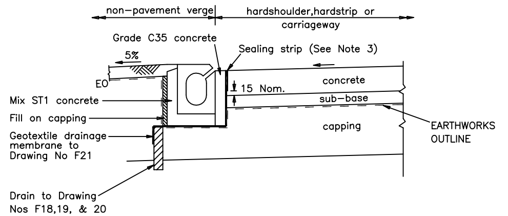
TYPE 25B (Rigid carriageway)
