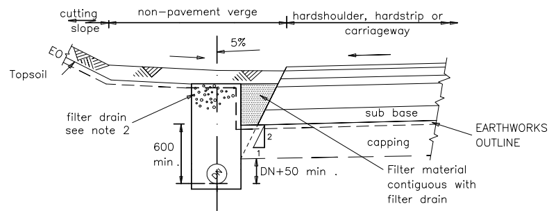
Type 1C (Flexible composite carriageway).
