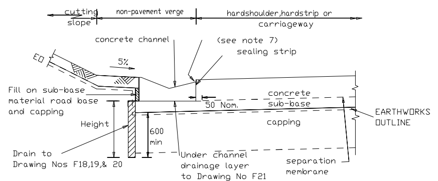
TYPE 2C (Channel formed on sub-base layer)
