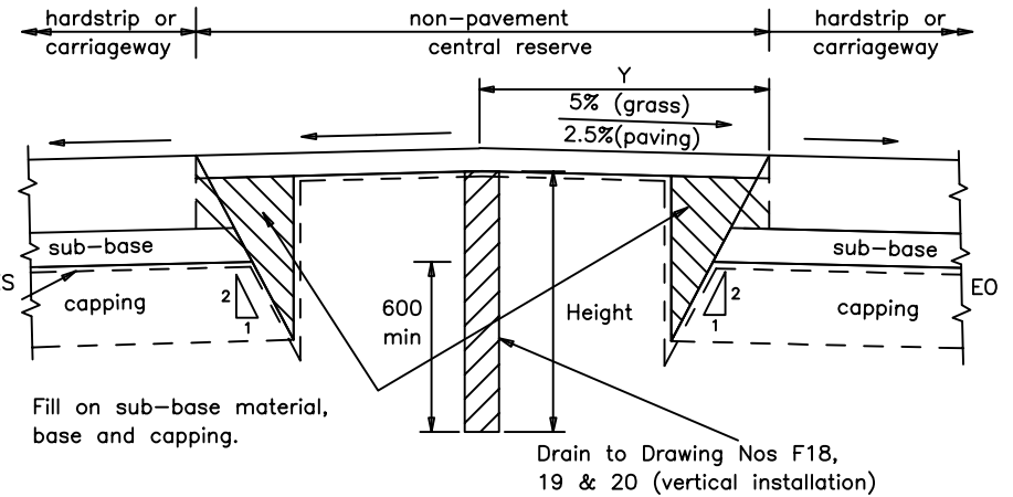
TYPE 16 (Drain in Raised Central Reserve)
