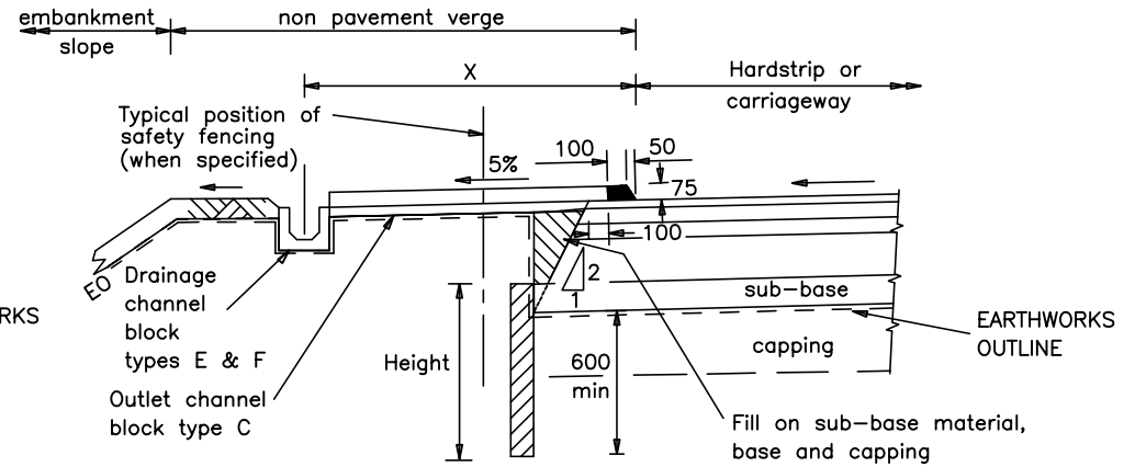
Type 21G (Flexible composite carriageway).
