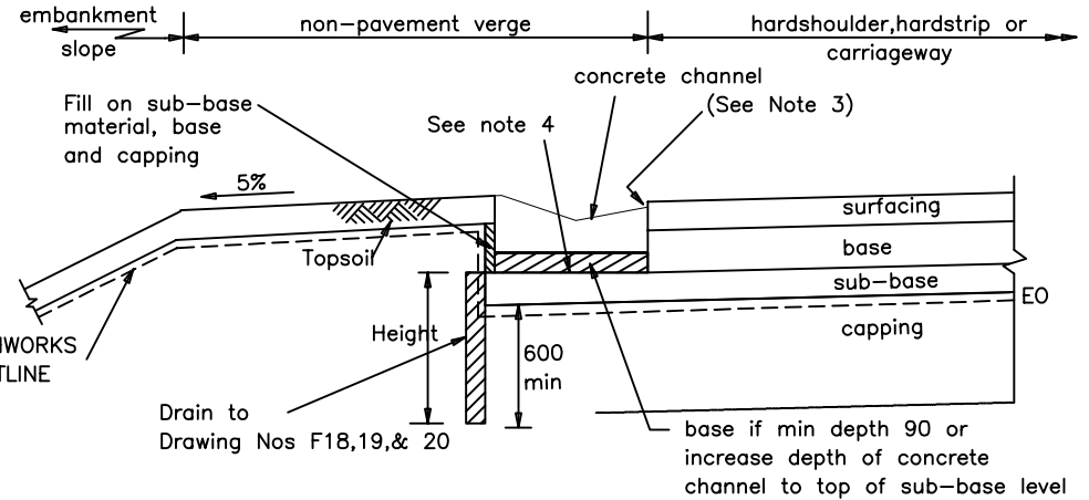
TYPE 23C (Channel formed on first base layer)
