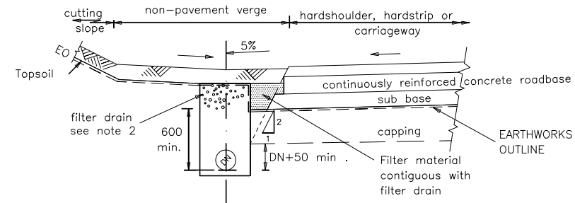
Type 1D (Rigid composite carriageway).
