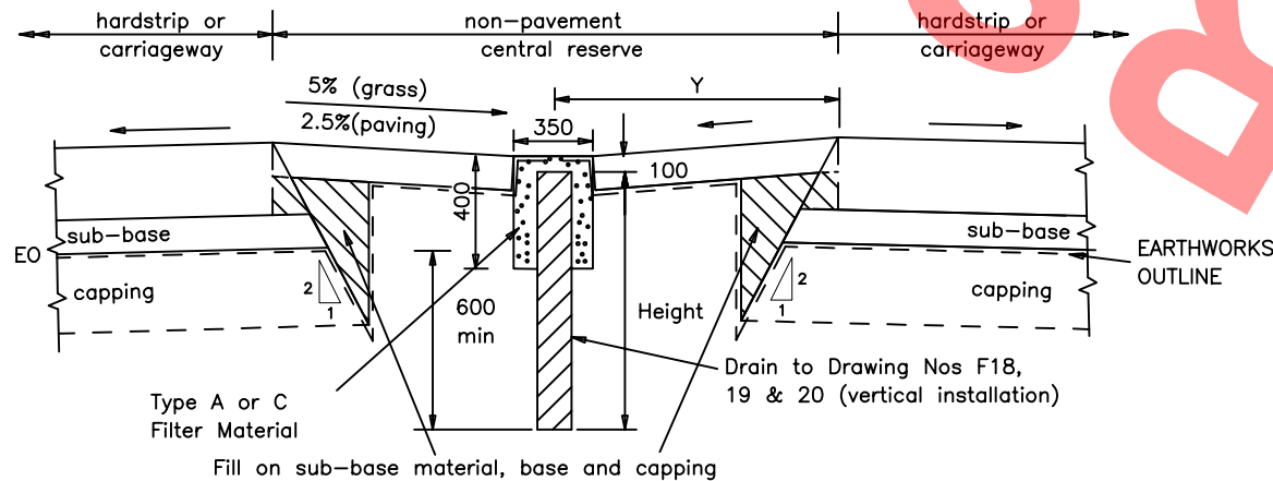
TYPE 15 (Drain in Dished Central Reserve)
