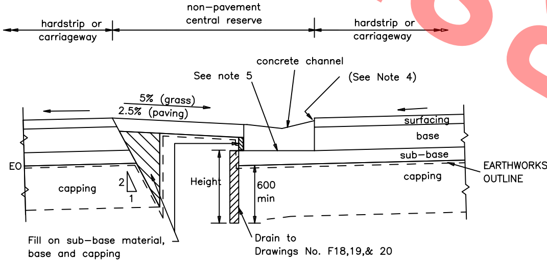
TYPE 13B (Channel formed on sub-base layer)
