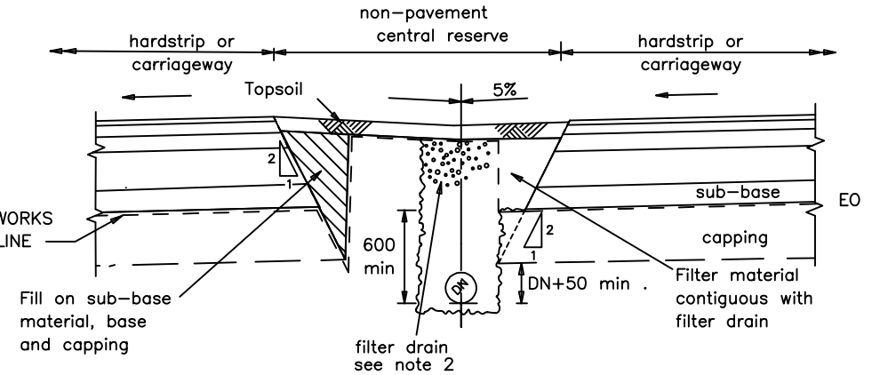
TYPE 11C (Flexible composite carriageway).
