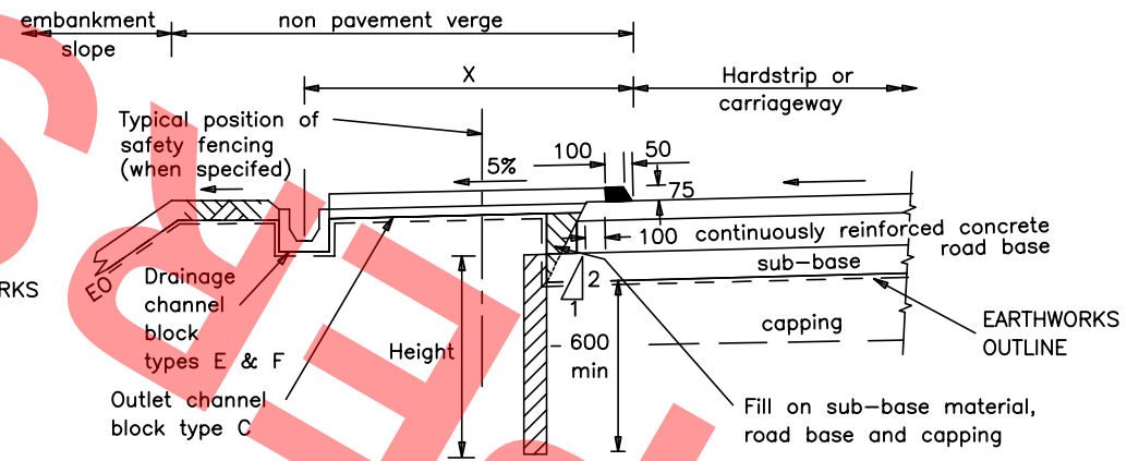
Type 21H (Rigid composite carriageway).
