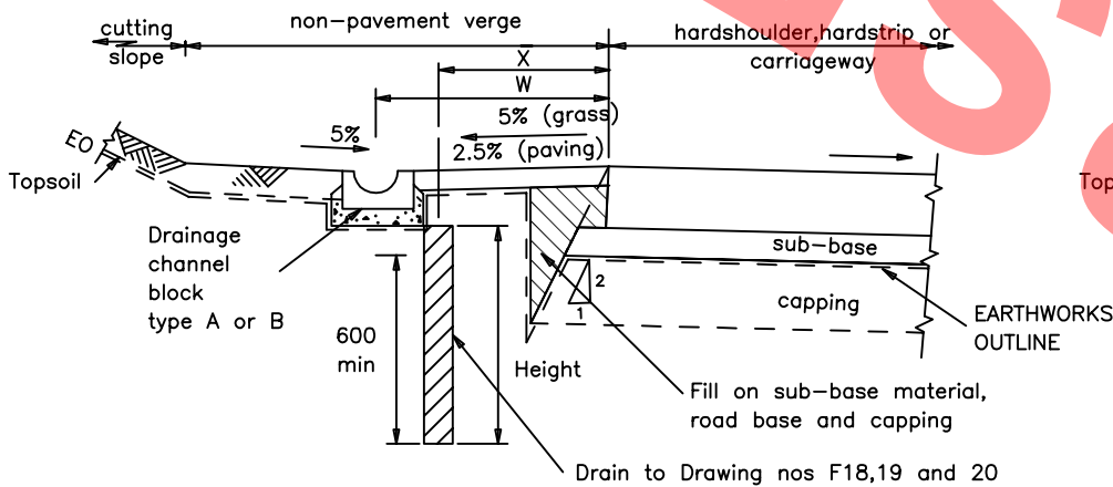
Type 4B (Rigid carriageway).
