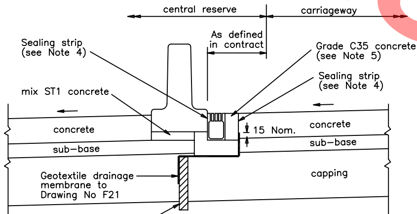
TYPE A2 (Proprietary precast system with rigid carriageway)
