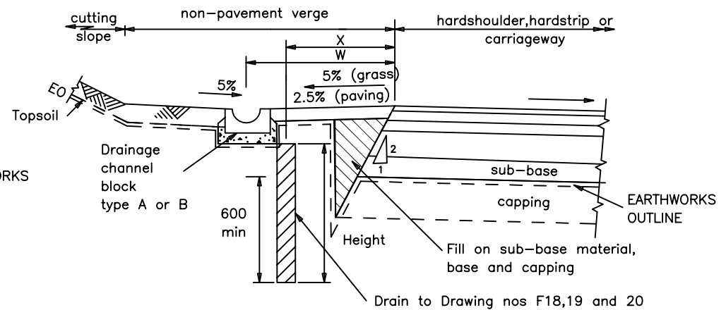
Type 4C (Flexible composite carriageway).
