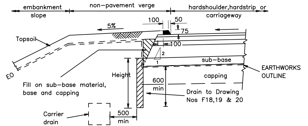
Type 21C (Flexible composite carriageway).
