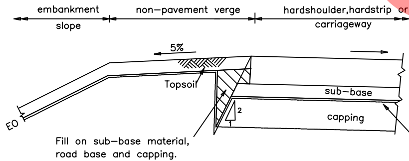
Type 24B (Rigid carriageway).
