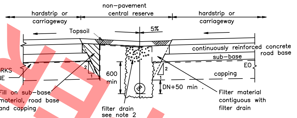
TYPE 11D (Rigid composite carriageway).
