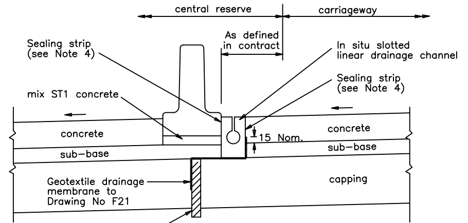
TYPE B1 (In situ system with rigid carriageway)
