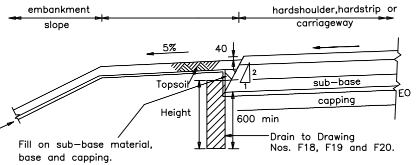
Type 24C (Flexible composite carriageway).
